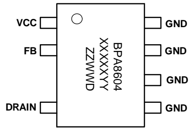
2 SOP-7
